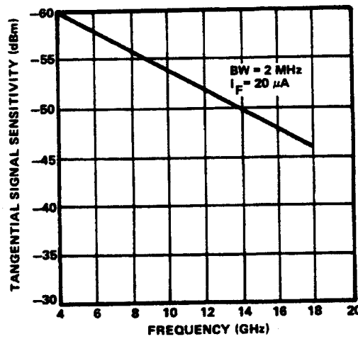
NOMINAL TANGENTIAL SIGNAL SENSITIVITY vs FREQUENCY
