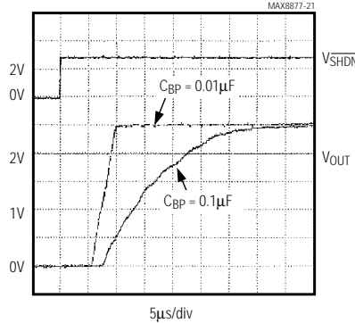
5µs/div MAX8877_EUK25, I_{LOAD} = 50mA
