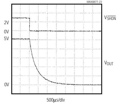
500µs/div MAX8878, NO LOAD
