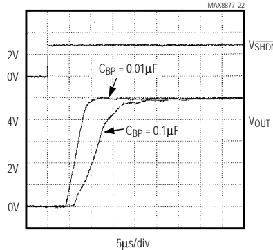
5µs/div MAX8877_EUK50, I_{LOAD} = 50mA
