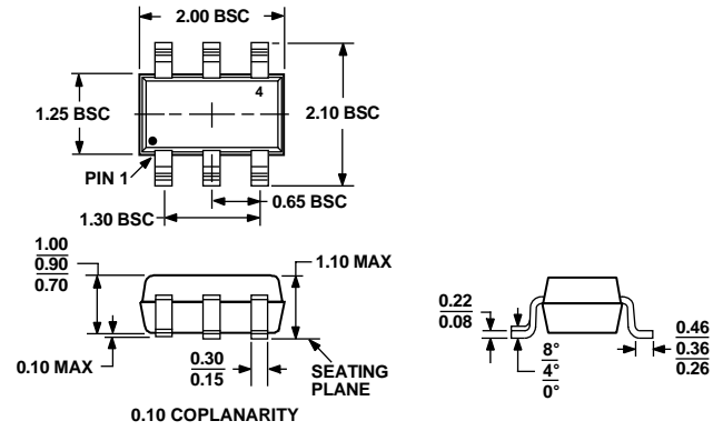
Figure 37. 6-Lead Plastic Surface Mount Package [SC70] (KS-6) Dimensions shown in millimeters
