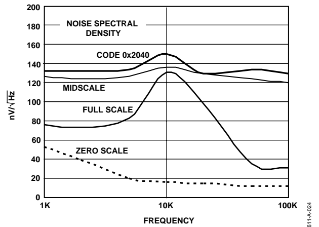
Figure 23. Noise Spectral Density
