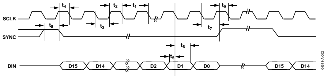
Figure 2. Timing Diagram
