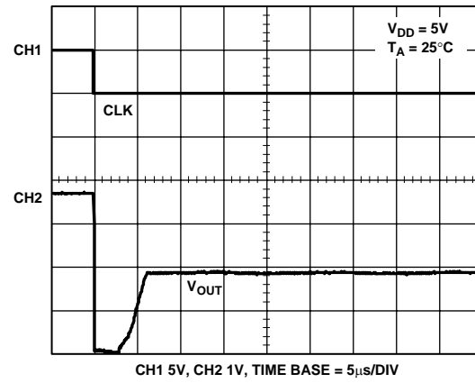
Figure 20. Exiting Power-Down
