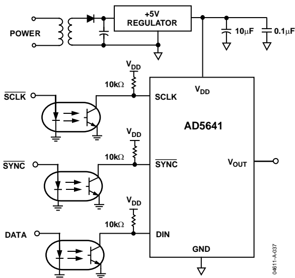
Figure 36. AD5641 with an Opto-Isolated Interface
