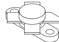
CASE 211-07, STYLE 2 MRF136
