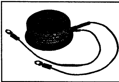
T820 Phase Control SCR 750-900 Amperes/100-2200 Volts
