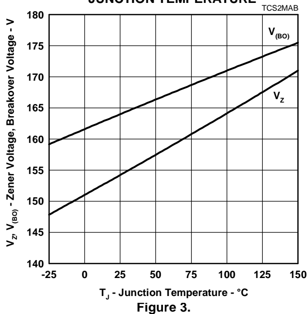
ZENER VOLTAGE & BREAKOVER VOLTAGE vs JUNCTION TEMPERATURE
