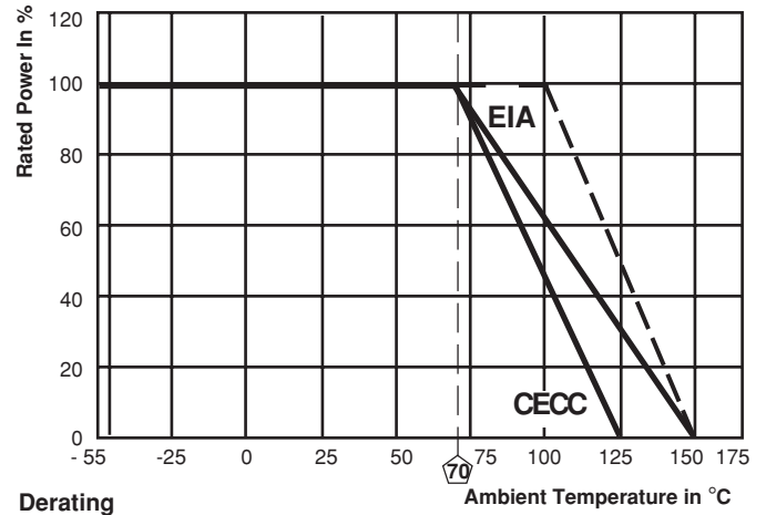
Derating
