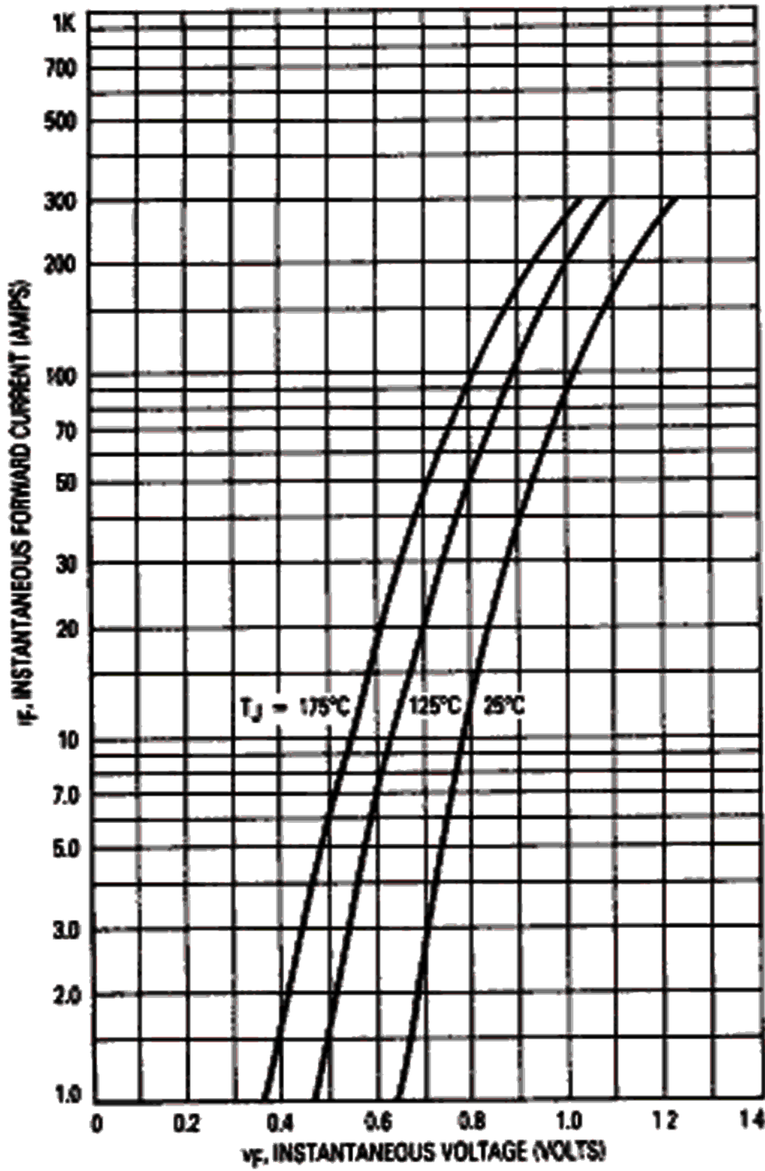
FIGURE 1 — FORWARD VOLTAGE
