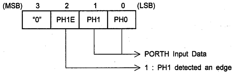
[READING PORTH INPUT DATA (PHY24)]
