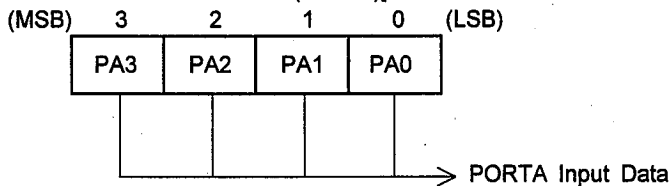
[READING PORTA INPUT DATA (PHY17)]
