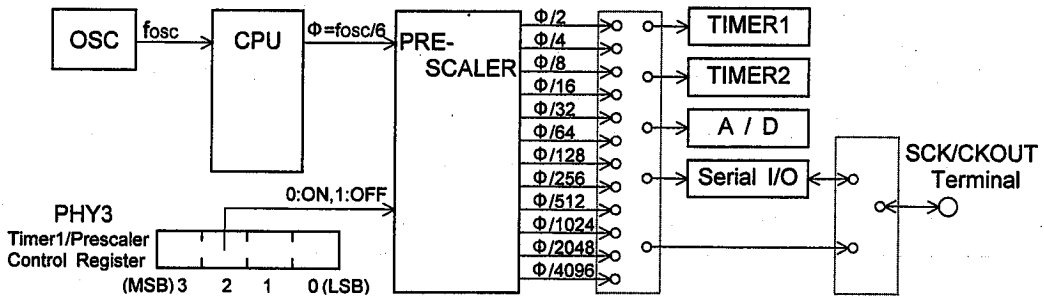
[AROUND THE PRESCALER BLOCK DIAGRAM]
