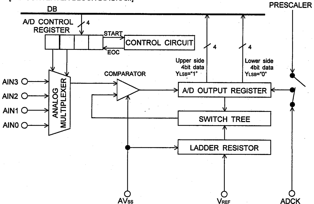
[A/D CONVERTER BLOCK DIAGRAM]
