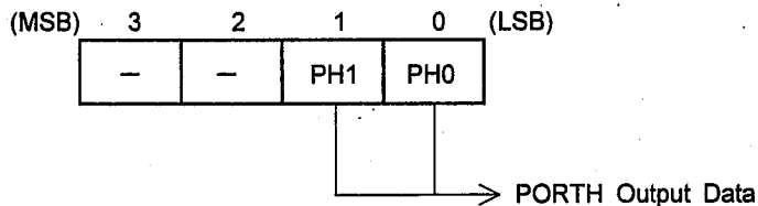
[WRITING PORTH OUTPUT DATA (PHY24)]
