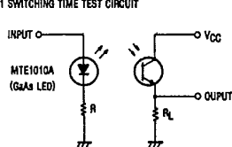
Fig. 1 SWITCHING TIME TEST CIRCUIT
