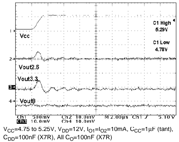
Figure 30 : Line Transient
