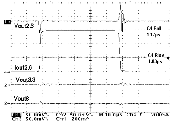
Figure 34 : Load Transient
