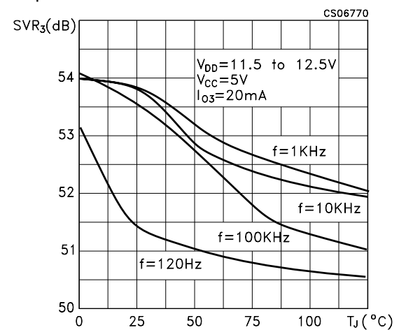
Figure 27 : Supply Voltage Rejection vs Temperature
