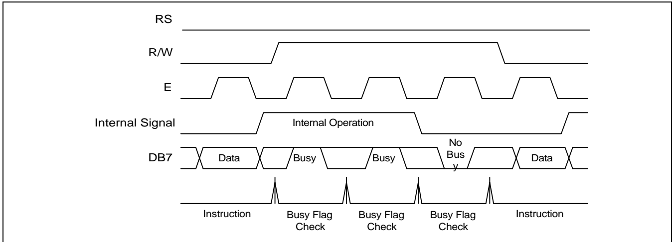
Figure 1. Example of 8-bit Bus Mode Timing Diagram
