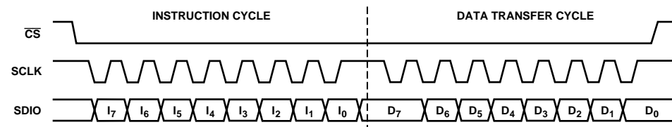
Figure 36. Serial Port Write Timing—Clock Stall High
