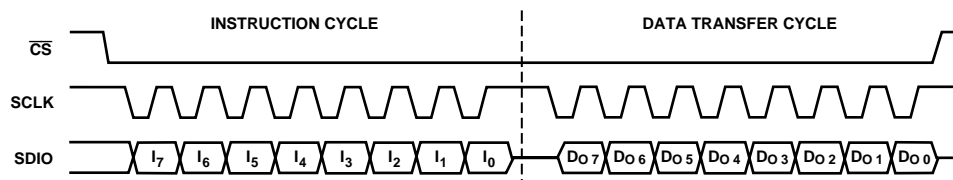
Figure 37. Two-Wire Serial Port Read Timing—Clock Stall High
