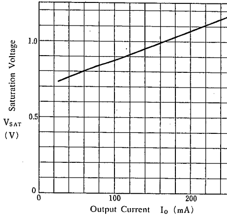
< Output Section > Saturation Voltage vs. Output Current (Ta=25°C)
