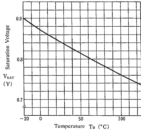
< Output Section > Saturation Voltage vs. Temperature (I o =100mA)
