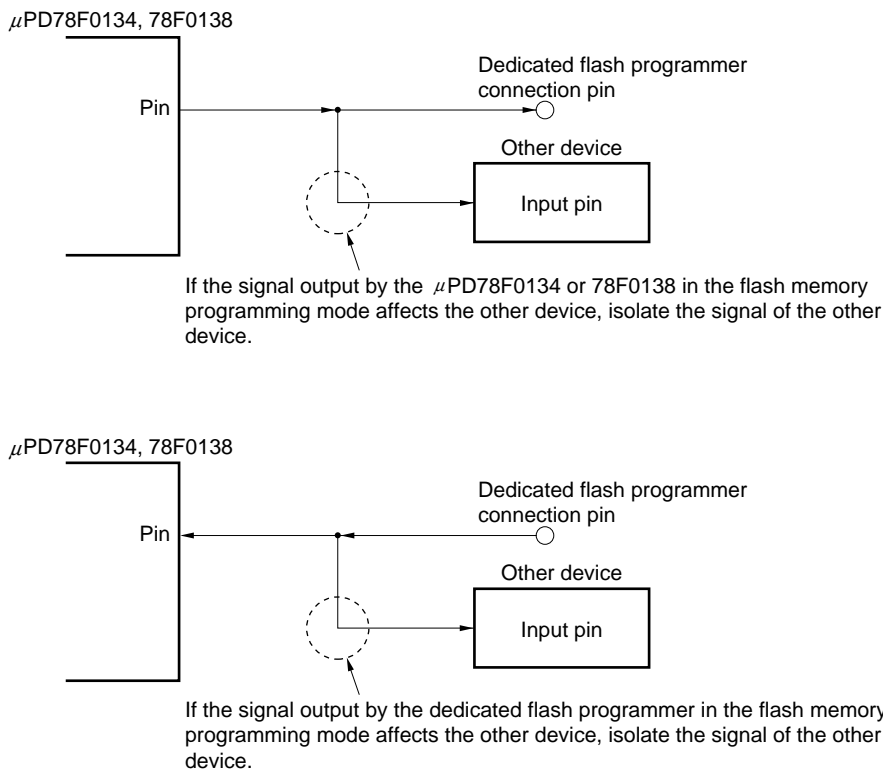
Figure 27-16. Malfunction of Other Device
