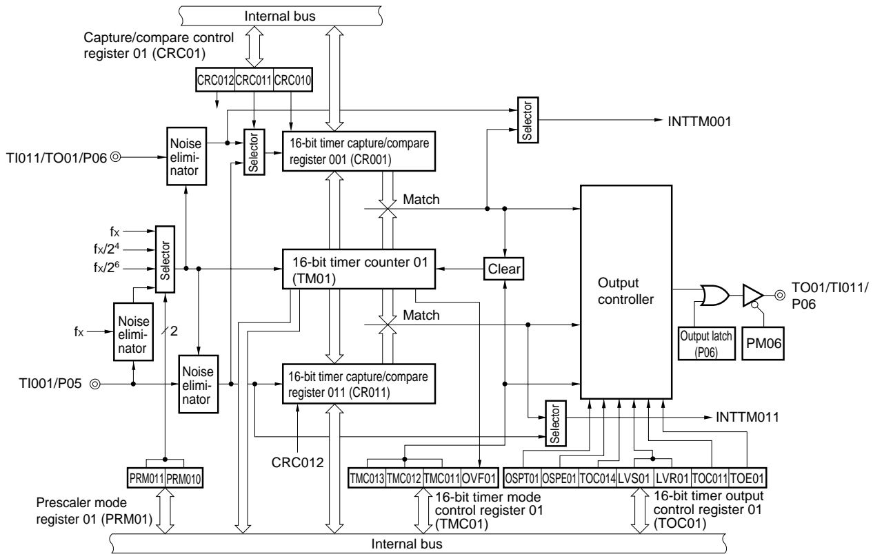
Figure 6-2. Block Diagram of 16-Bit Timer/Event Counter 01 (μPD780133, 780134, 78F0134, 780136, 780138, 78F0138 Only)
