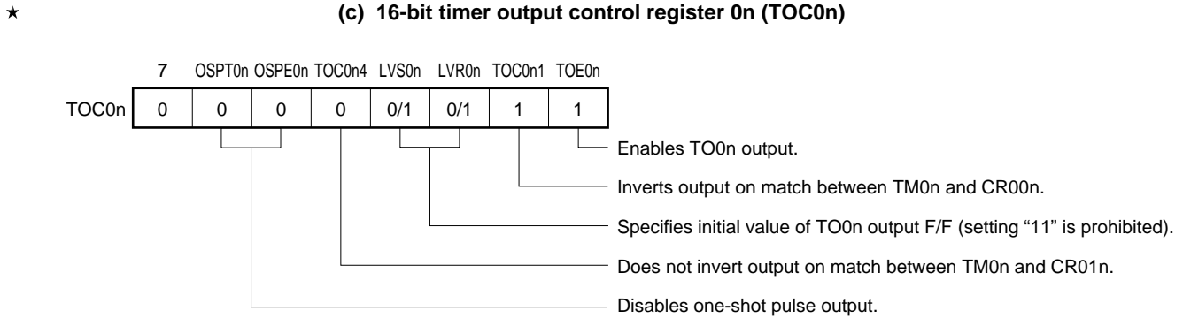
Figure 6-34. Control Register Settings in Square-Wave Output Mode (2/2)
