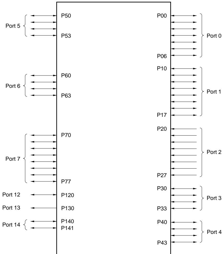
Figure 4-1. Port Types
