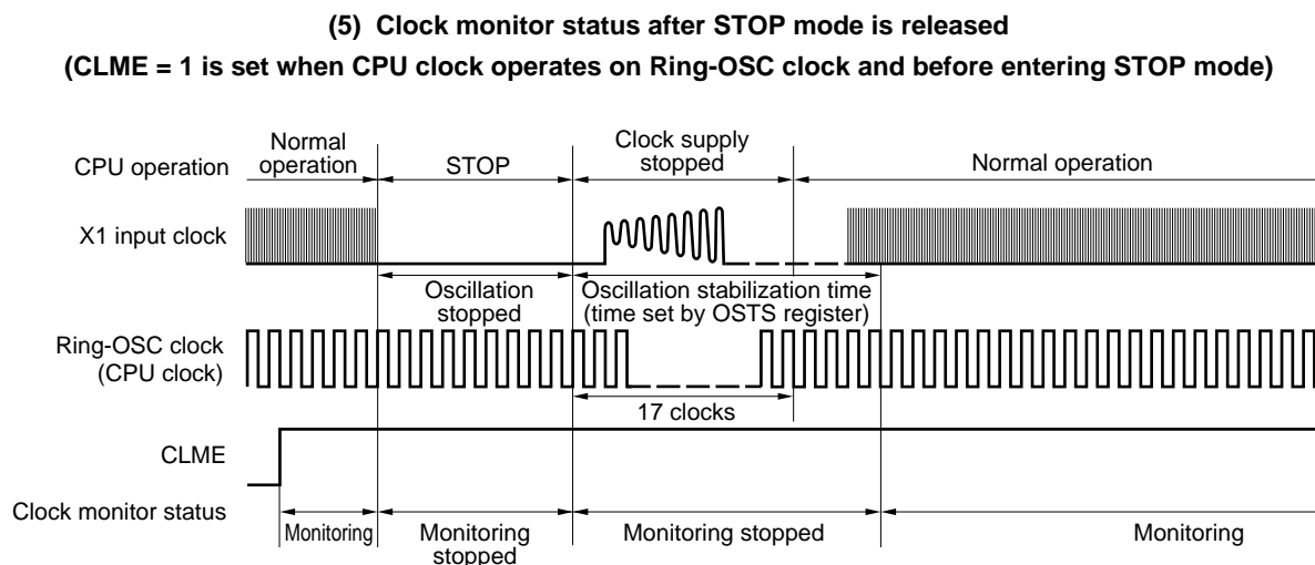
Figure 21-3. Timing of Clock Monitor (3/4)
