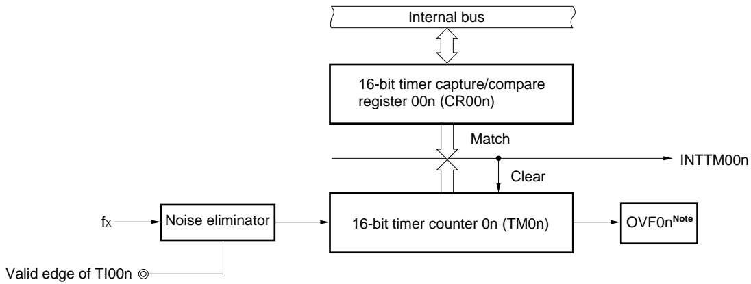
Figure 6-32. Configuration Diagram of External Event Counter
