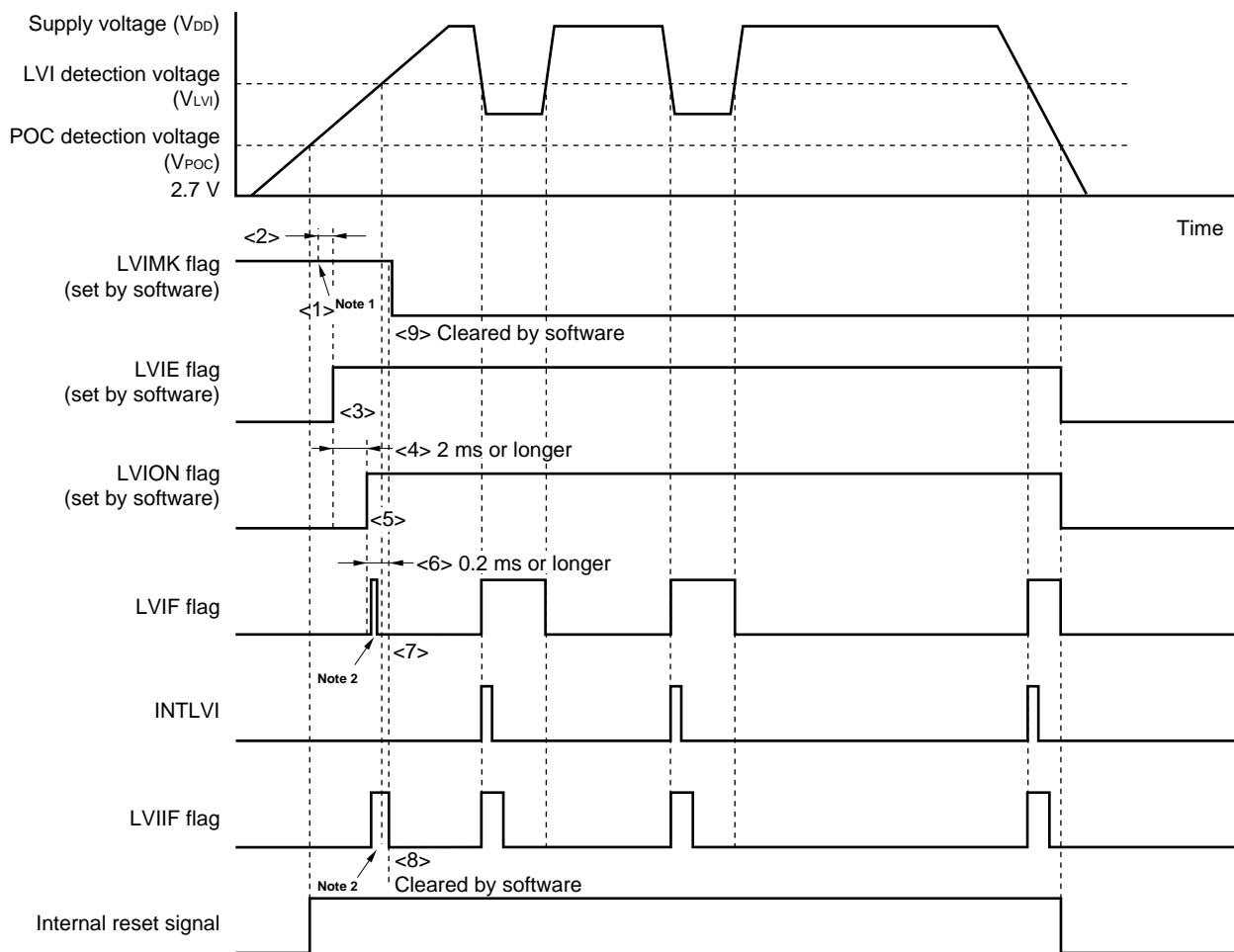
Figure 23-5. Timing of Low-Voltage Detector Interrupt Signal Generation
