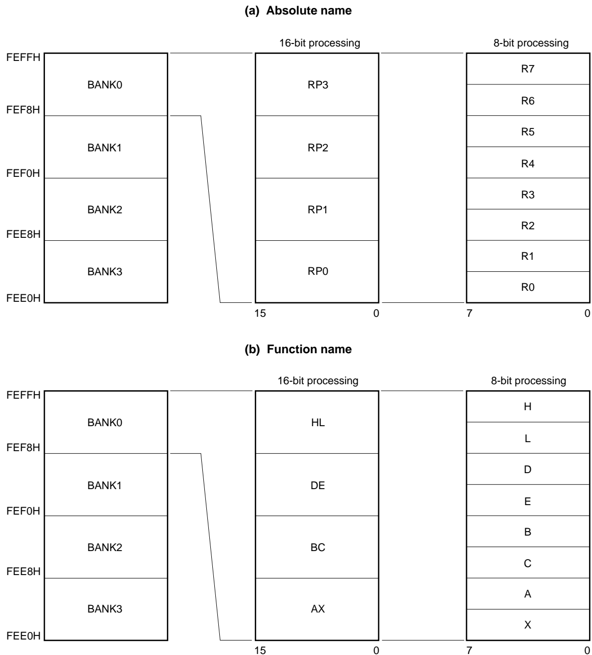
Figure 3-22. Configuration of General-Purpose Registers
