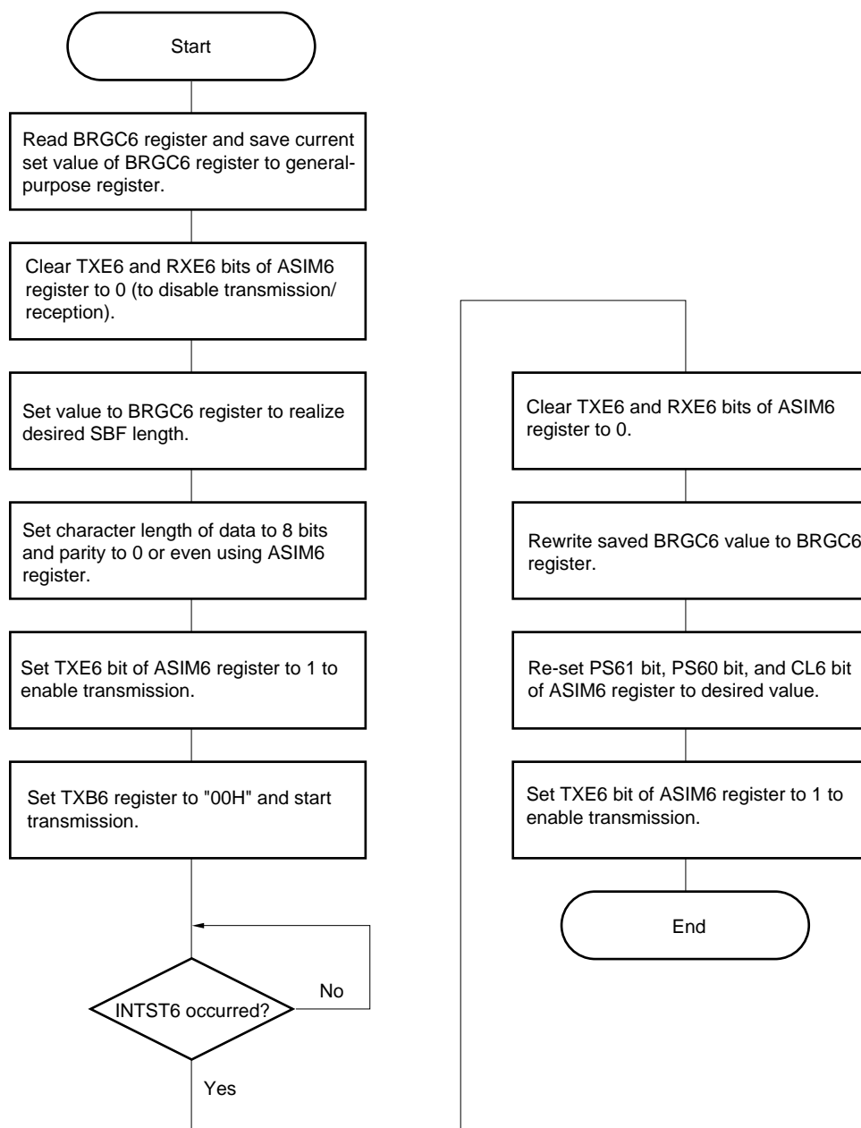
Figure 14-23. SBF Transmission
