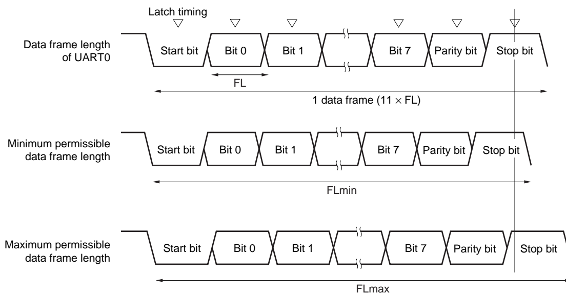
Figure 13-12. Permissible Baud Rate Range During Reception
