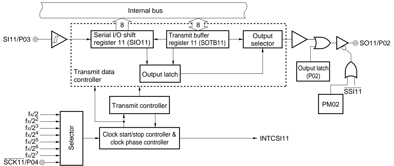
Figure 15-2. Block Diagram of Serial Interface CSI11
