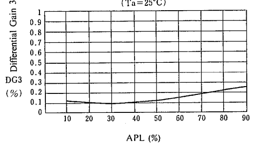
Differential Gain 3 vs. APL
