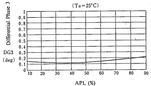
Differential Phase 3 vs. APL
