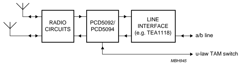
b. Base with analog interface and echo cancellation; up to 6 portables can be handled.
