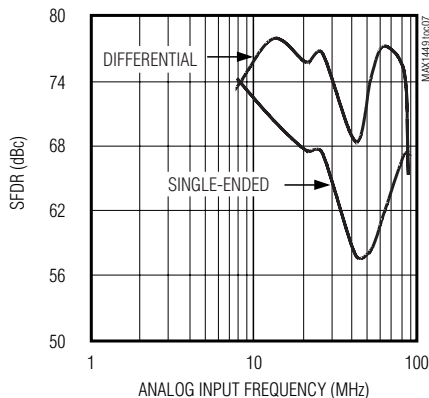
SPIRIOUS-FREE DYNAMIC RANGE vs. ANALOG INPUT FREQUENCY
