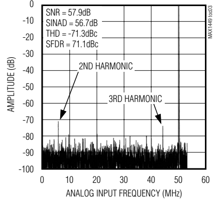
UNDERSAMPLING FFT PLOT ( f_{IN} = 50.12MHz , 8192-POINT FFT, DIFFERENTIAL INPUT)
