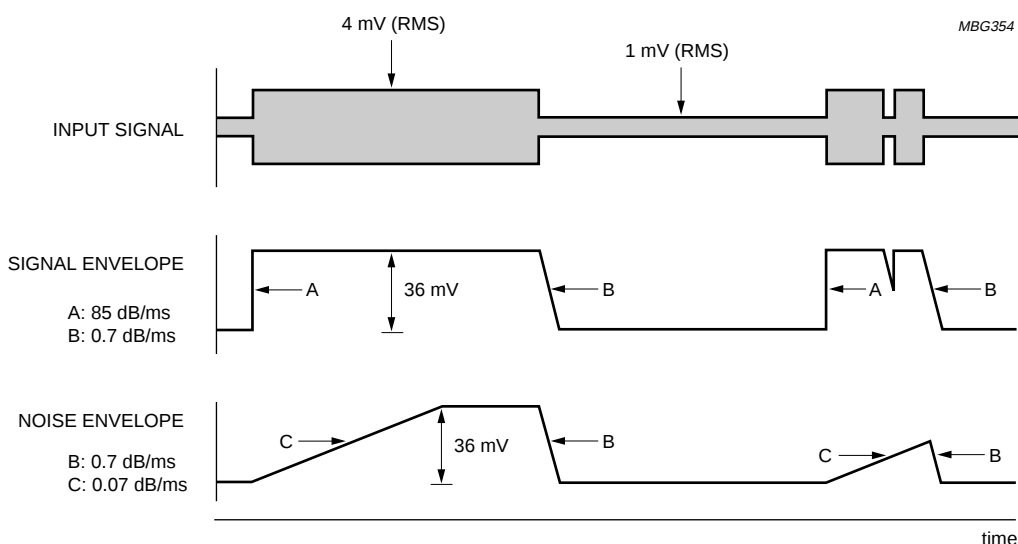
Fig.11 Signal and noise envelope waveforms.
