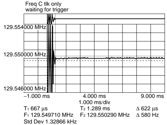
Lock up time (PLLPS mode to Lock, f_{vco} within \pm 300 Hz)
