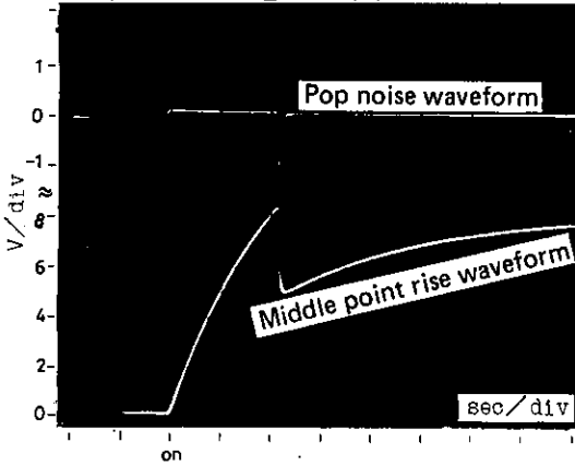
Pop noise waveform at the time of power switch ON ( V_{CC} = 16V, R_L = 8\Omega , quiescent)
