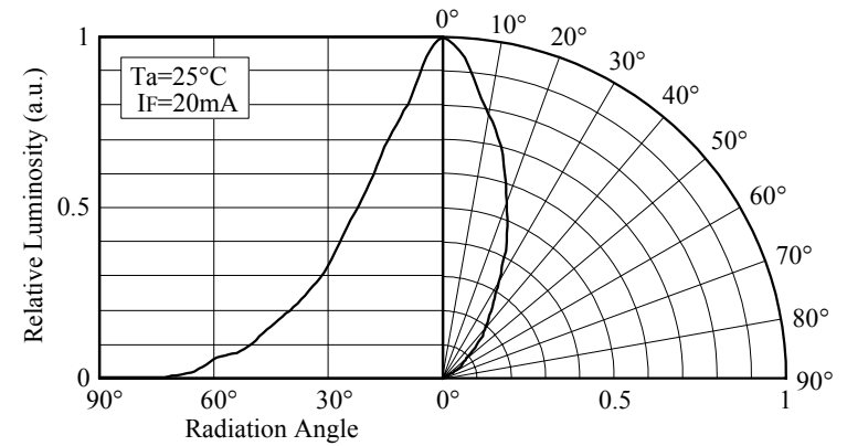
■ Directivity (NSPB320BS)
