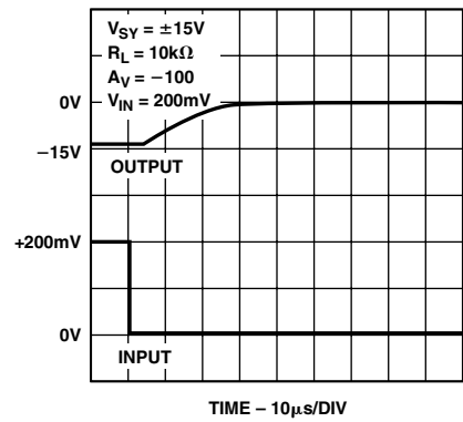
TPC 12. Positive Overvoltage Recovery
