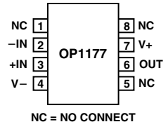
8-Lead SOIC (R-Suffix)
