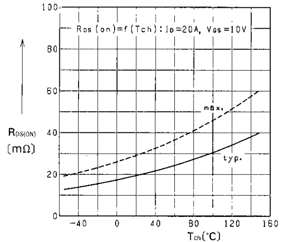
On-State Resistance vs. T_{ch}
