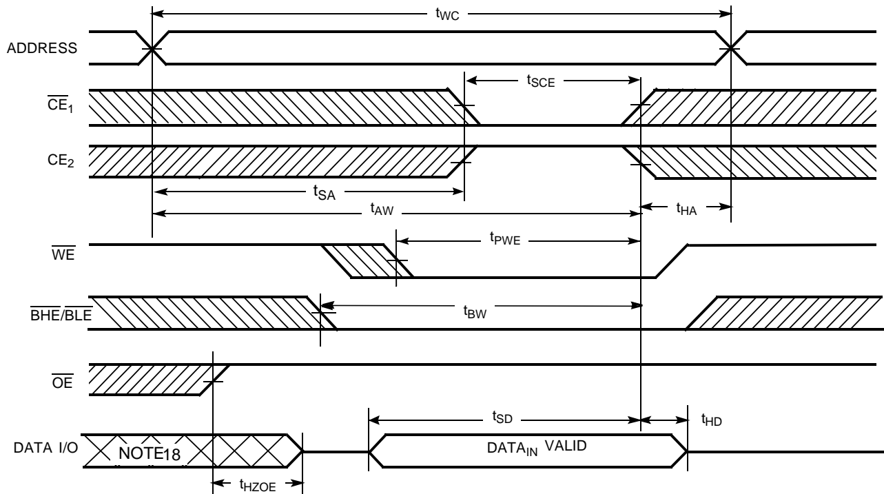
Write Cycle No. 2 ( \overline{CE}_1 or \overline{CE}_2 Controlled) [12, 16, 17]
