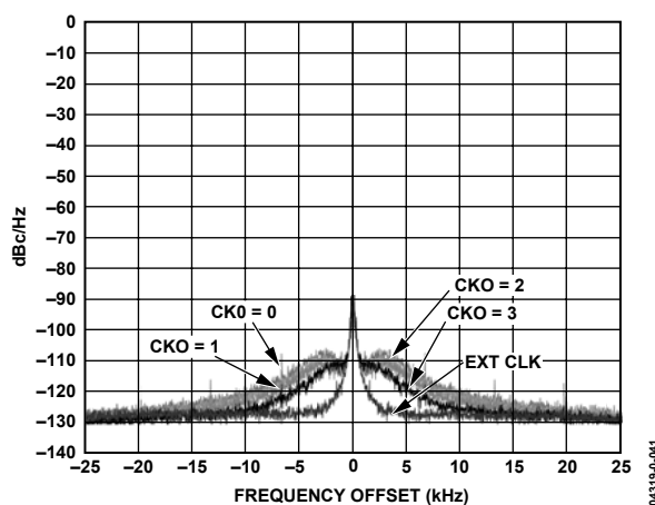
Figure 41. CLK Phase Noise vs. I_{BIAS} Setting ( CKO ) ( IF = 73.35 \text{ MHz} , IF = 71.1 \text{ MHz} , IFIN = -31 \text{ dBm} , f_{CLK} = 18 \text{ MHz} , f_{REF} = 16.8 \text{ MHz} ) ( CLK SYN Settings: CKI = 7 , CLR = 56 , and CLN = 60 with f_{REF} = 300 \text{ kHz} )
