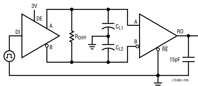
Figure 3. Driver/Receiver Timing Test Circuit
