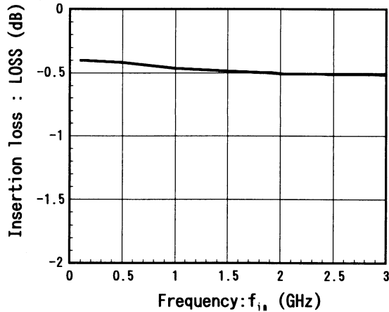
(PC-P2) Insertion loss vs. Frequency ( V_{cTX}=0V/2.7V , P_{iA}=22dBm )
