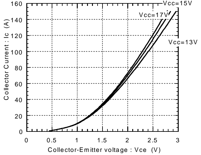
Collector current vs. Collector-Emittor voltage T j =125°C
