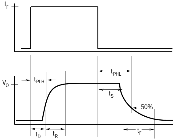
Figure 2. Non-saturated switching timing
