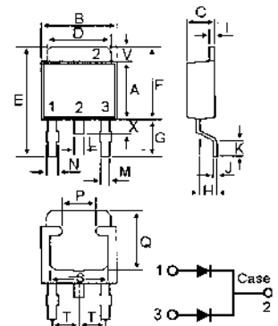
TO-252AA (DPAK)
