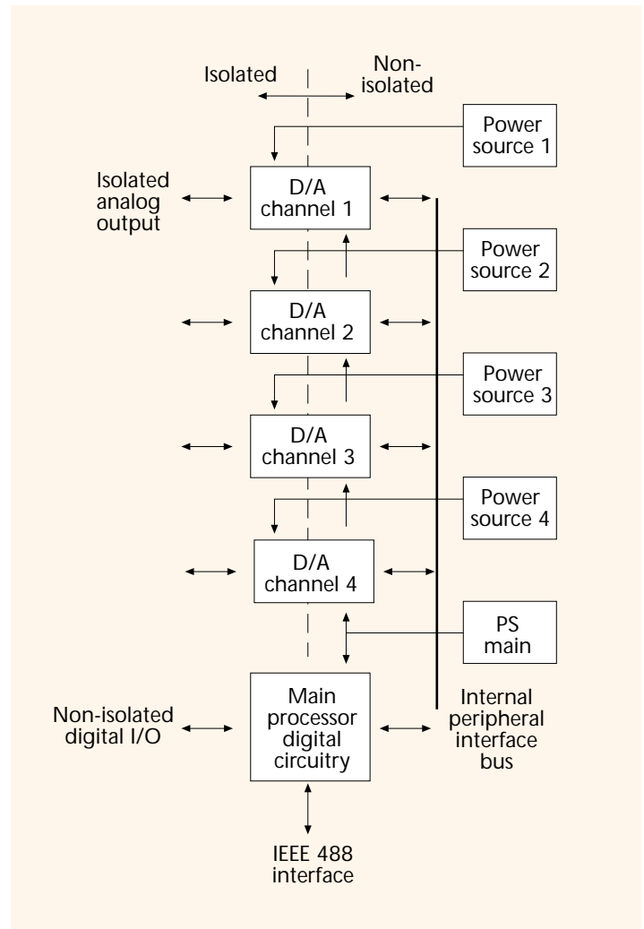
Each DAC488HR output port features a separate microprocessor and buffer memory for independent waveform management
