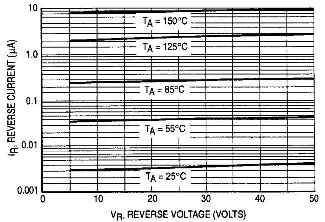
Figure 3. Leakage Current
