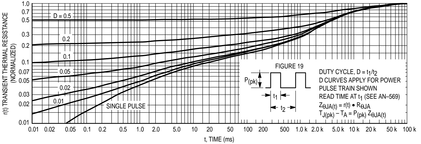
Figure 17. Thermal Response
