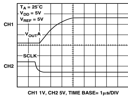
Figure 19. Half-Scale Settling (1/4 to 3/4 Scale Code Change)
