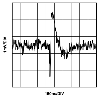
Figure 26. DAC-to-DAC Crosstalk
