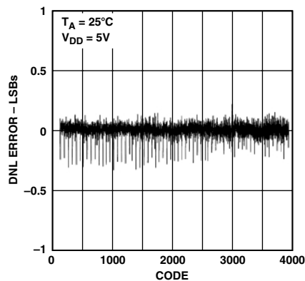
Figure 9. AD5324 Typical DNL Plot
