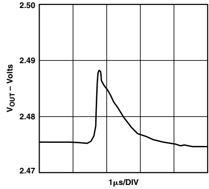
Figure 23. AD5324 Major-Code Transition Glitch Energy
