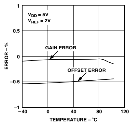
Figure 12. AD5304 Offset Error and Gain Error vs. Temperature
