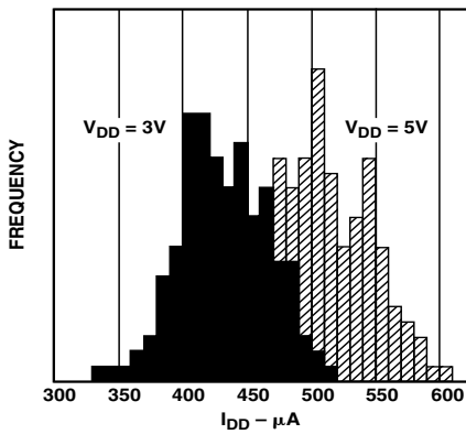
Figure 22. I_{DD} Histogram with V_{DD} = 3V and V_{DD} = 5V
