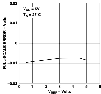
Figure 25. Full-Scale Error vs. V_{REF}
