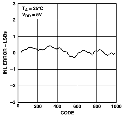
Figure 5. AD5314 Typical INL Plot
