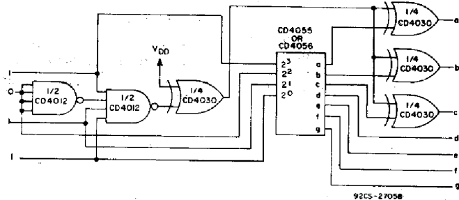
Fig. 21 — Conversion of "H" display to "F" display.
