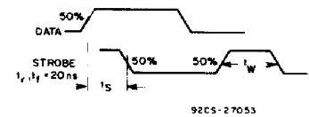
Fig. 15 — Data setup time and strobe pulse duration.
