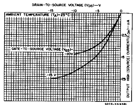
Fig. 13 - Minimum p-channel output high (source) current characteristics.
