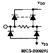
Fig.2 - CD4055B functional diagram.
