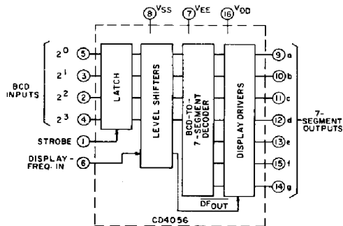
Fig.3 - CD4056B functional diagram.
