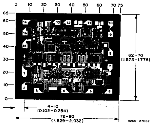
Dimensions and pad layout for CD4054BH.
