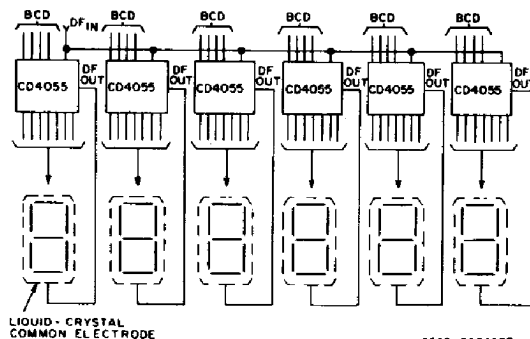
Fig. 16 — Clock display: V_{DD} = 0\text{ V} , V_{SS} = -5\text{ V} , V_{EE} = -15\text{ V} , DF_{IN} = 30\text{ Hz} square wave.
