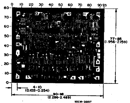
Dimensions and pad layout for CD4056BH
