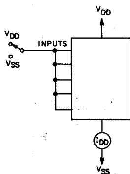
Fig. 10 - Quiescent device current test circuit.
