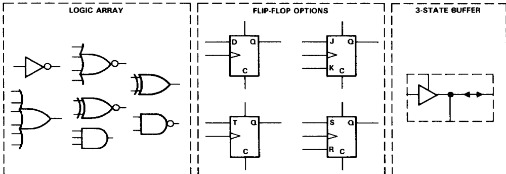
FIGURE 1. MACROCELL COMPONENTS
