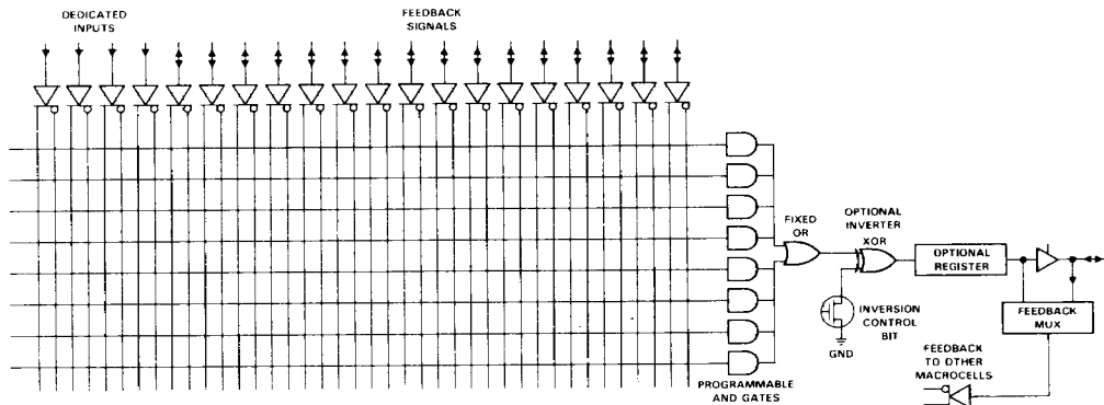
FIGURE 11. EPLD MACROCELL
