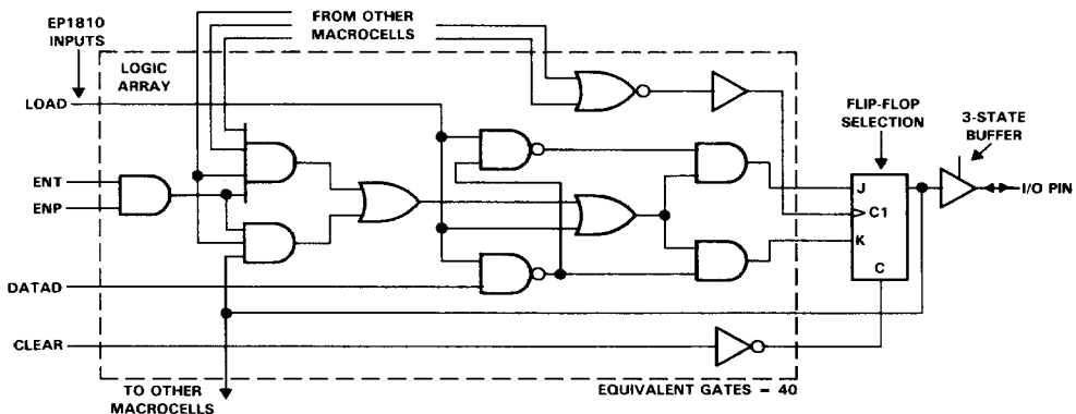
FIGURE 2. SAMPLE CIRCUIT
