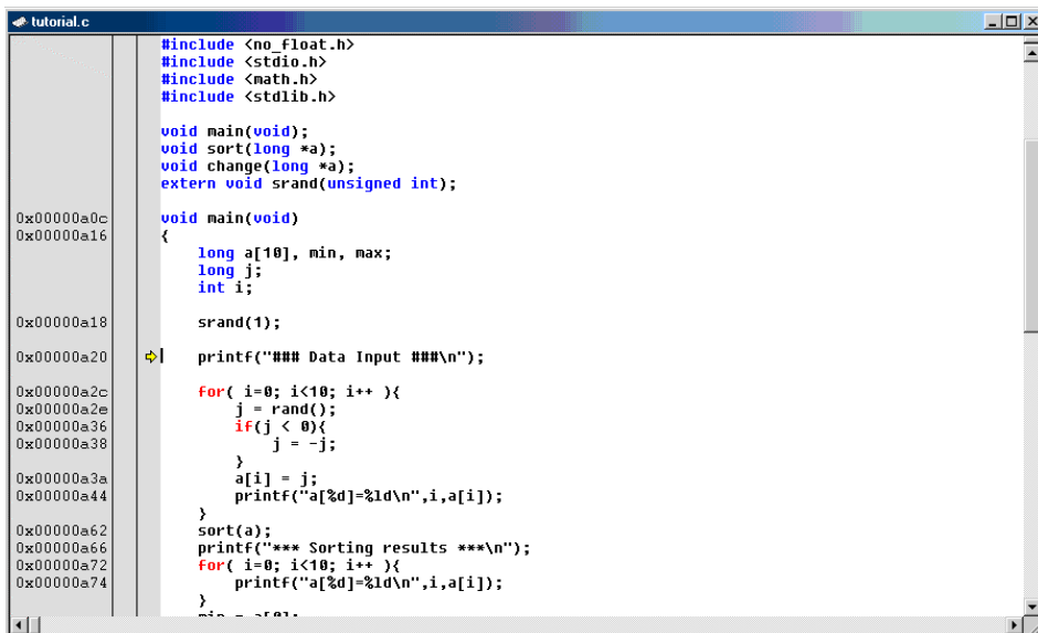
Figure 3.6: Source window and address column
