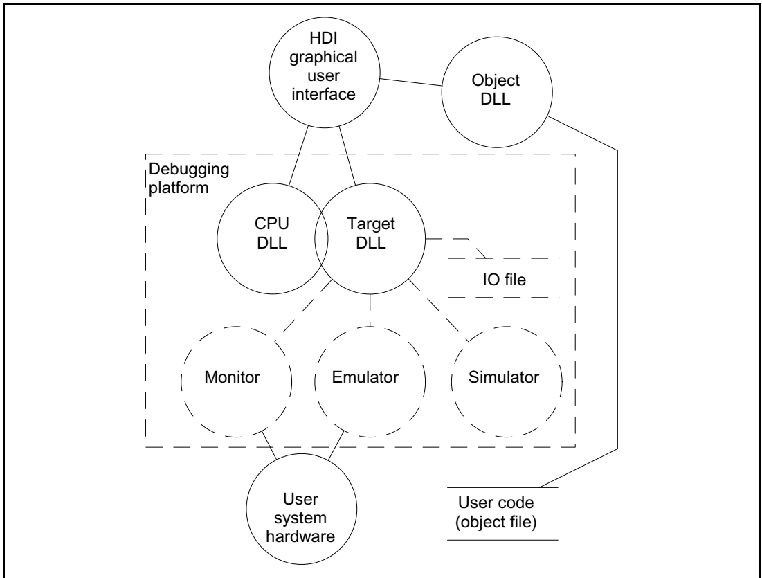
Figure A.1 HDI System Modules
