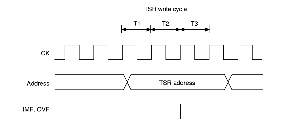
Figure 10.57 Timing of Status Flag Clearing
