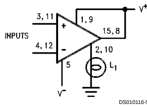
Driving Ground-Referred Load
