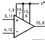
Increasing Input Stage Current*
