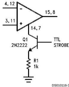
Strobing
