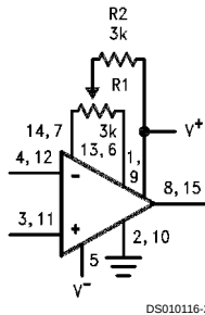
Offset Balancing
