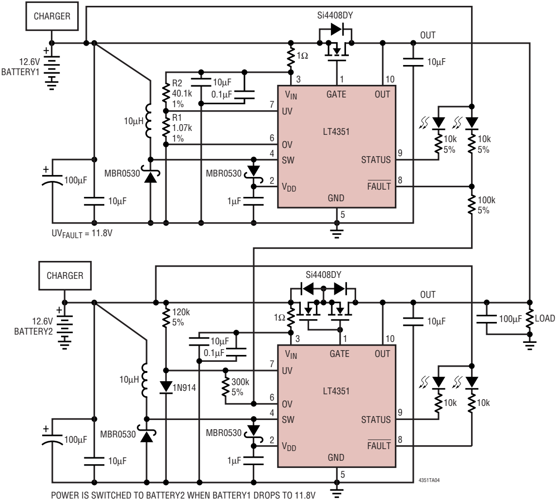
Primary Battery with Secondary Battery Backup
