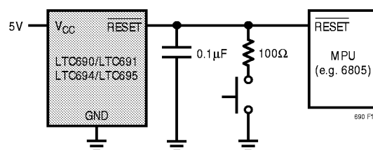
Figure 13. The External Push-Button Reset
