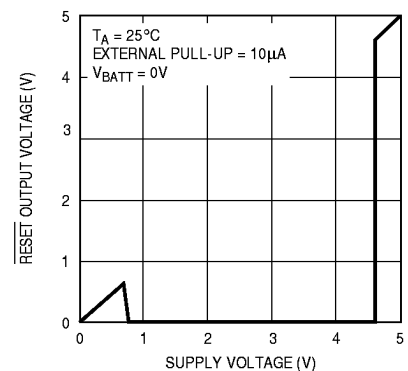
\overline{\text{RESET}} Output Voltage vs Supply Voltage
