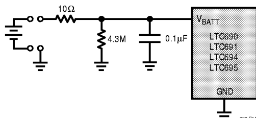
Figure 4. 10\Omega/0.1\mu\text{F} Combination Eliminates Inductive Overshoot and Prevents Spurious Resets During Battery Replacement
