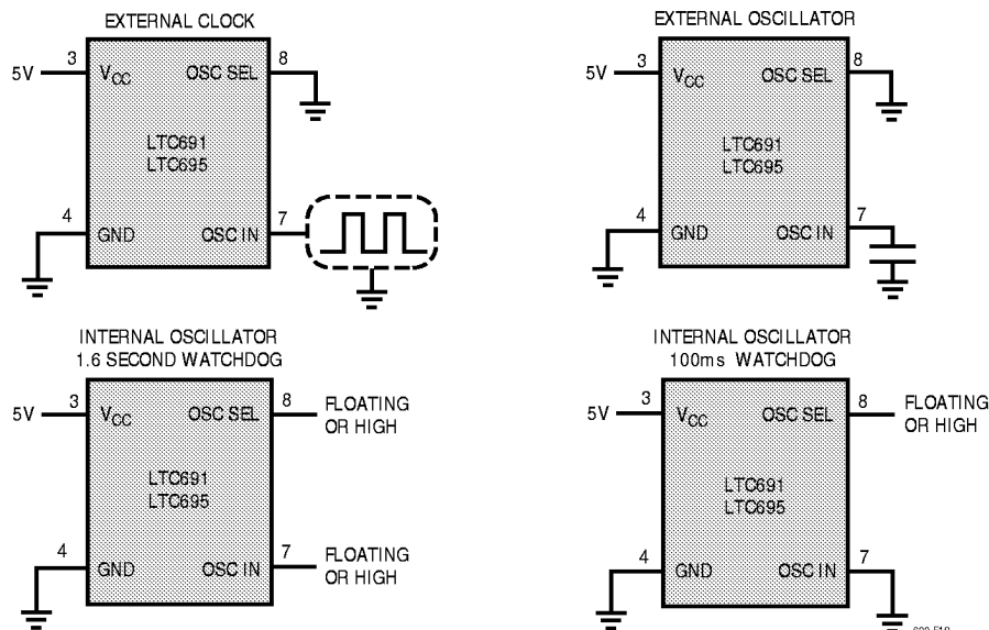
Figure 12. Oscillator Configurations
