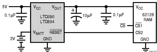
Figure 7. Write Protect for RAM with LTC690 or LTC694
