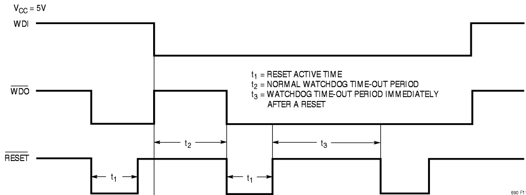
Figure 11. Watchdog Time-Out Period and Reset Active Time
