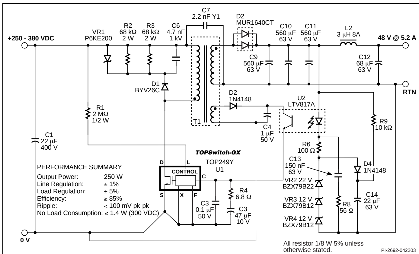
Figure 43. 250 W, 48 V Power Supply using TOP249.
