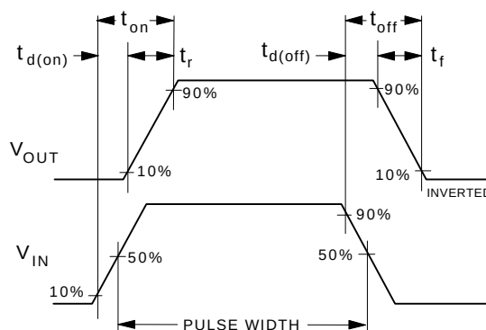
Figure 12. Switching Waveforms.
