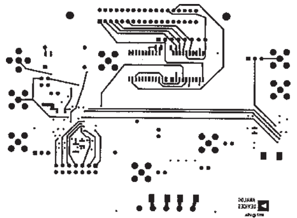
d. Layer 4 (Bottom) – Signal Routing
