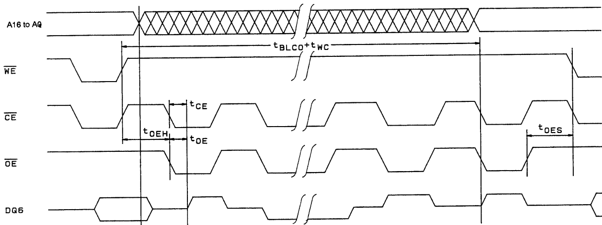
Figure 5 Toggle Bit
