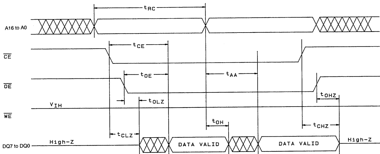
Figure 1 Read Cycle
