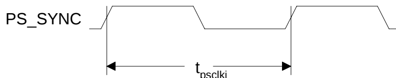
Figure 5. PS_SYNC Timings
