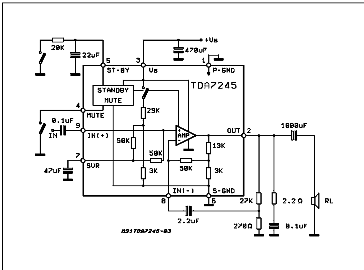
Figure 2: Schematic Diagram
